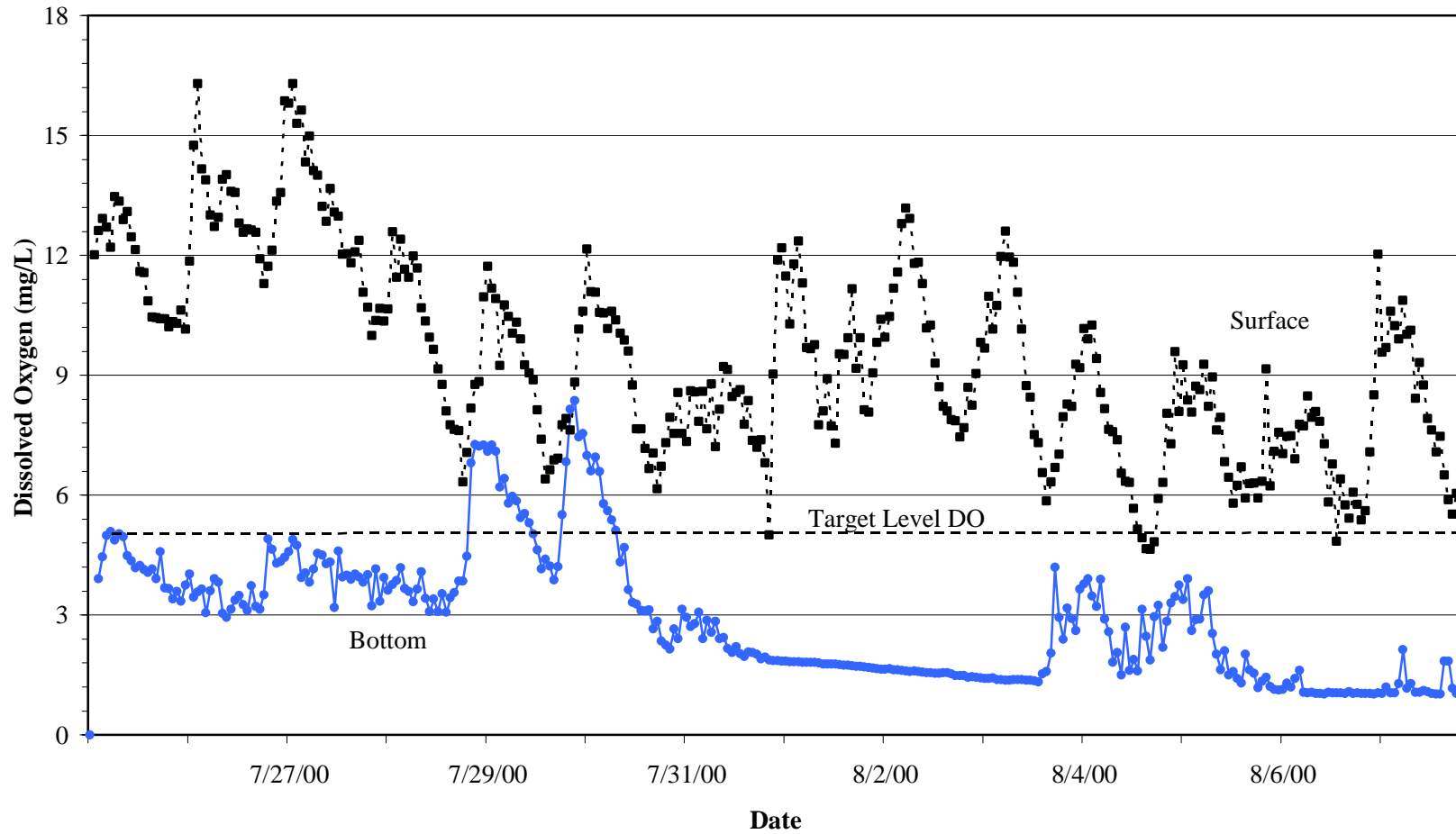
Figure E-2. Monitoring Results at Station W-M328.7B during Summer 2000
