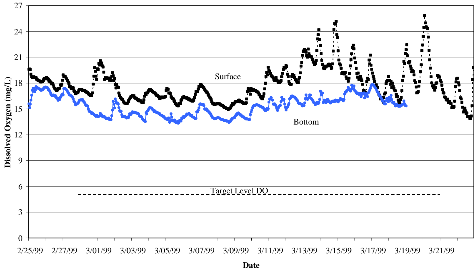
Figure E-1. Monitoring Results at Station W-M328.7B during Winter 1999
